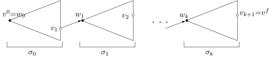
Fig. 9. Path decomposition in local-choice HMSC.
