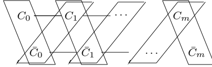
Fig. 6. TM computation.
